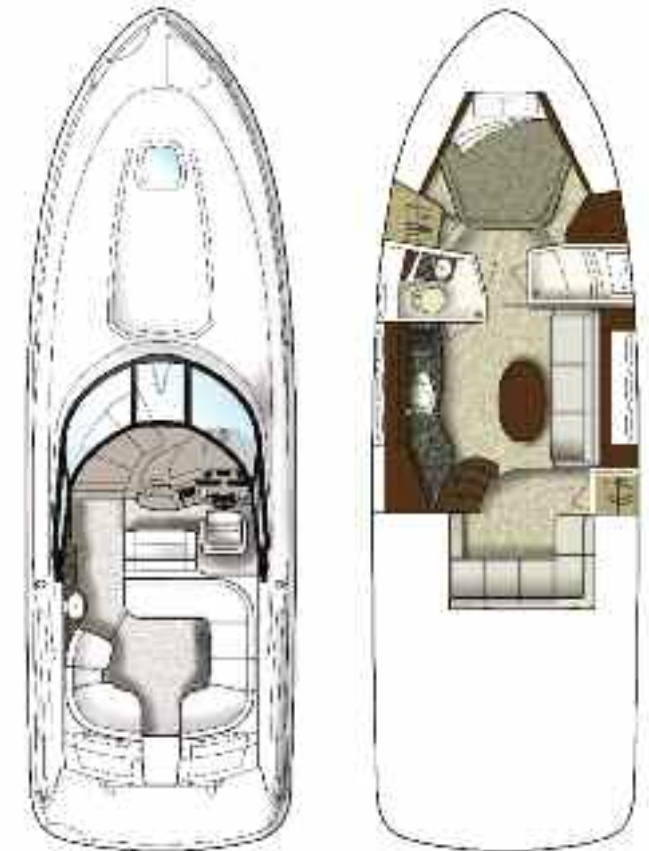
Cockpit Layout
